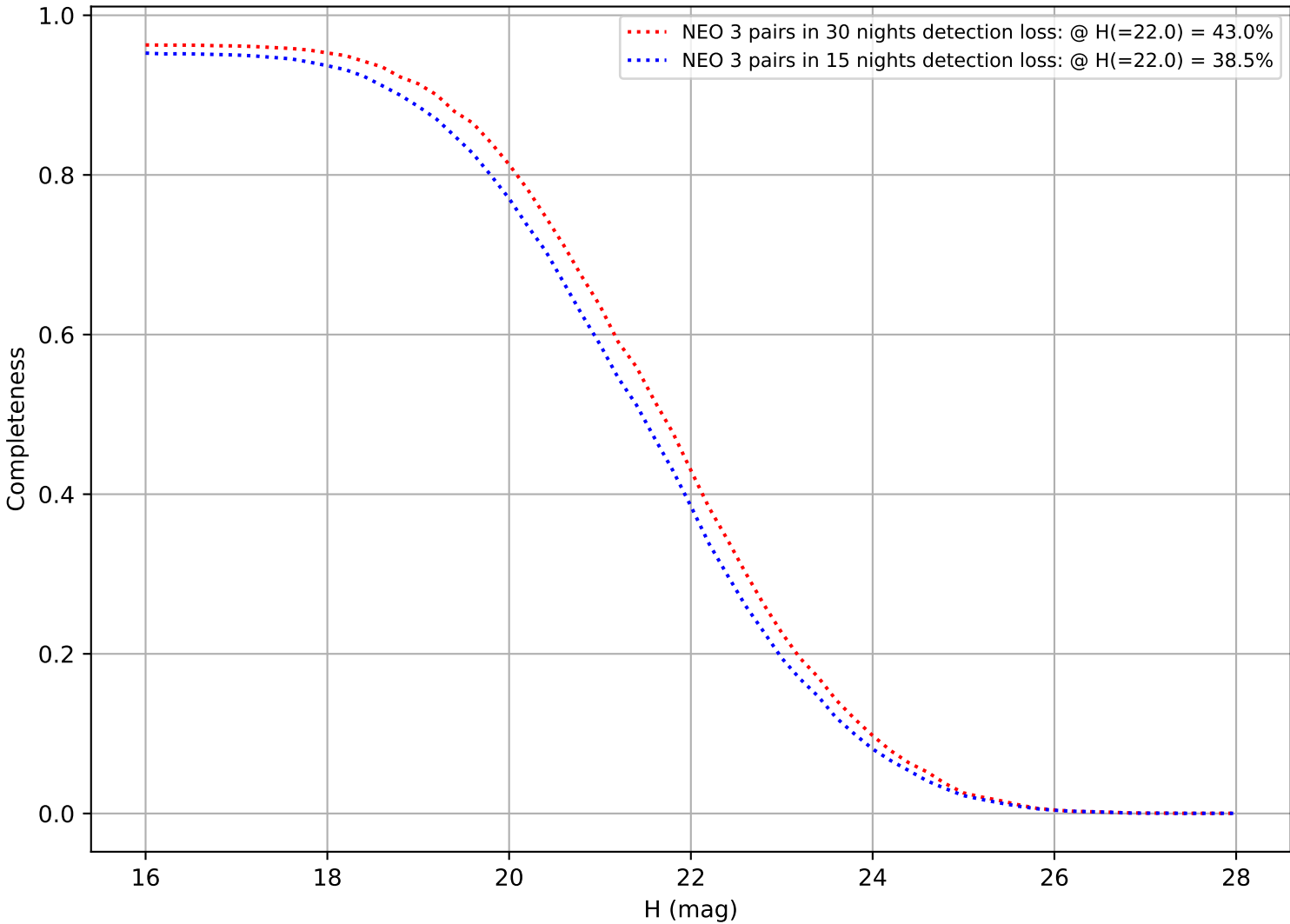
weather_cloudso2v3.5_10yrs: DifferentialCompleteness
