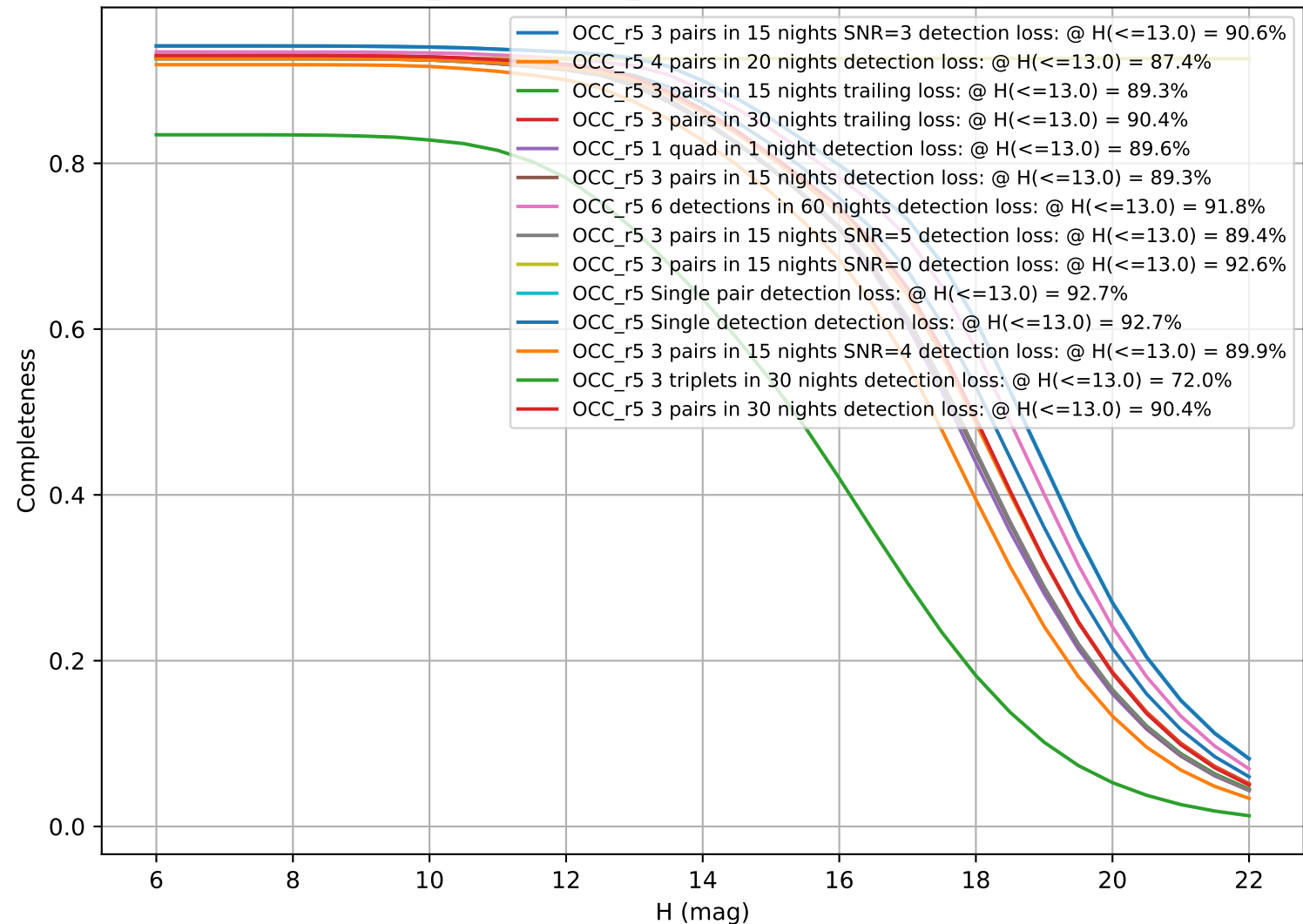
weather_cloudso2v3.5_10yrs: CumulativeCompleteness
