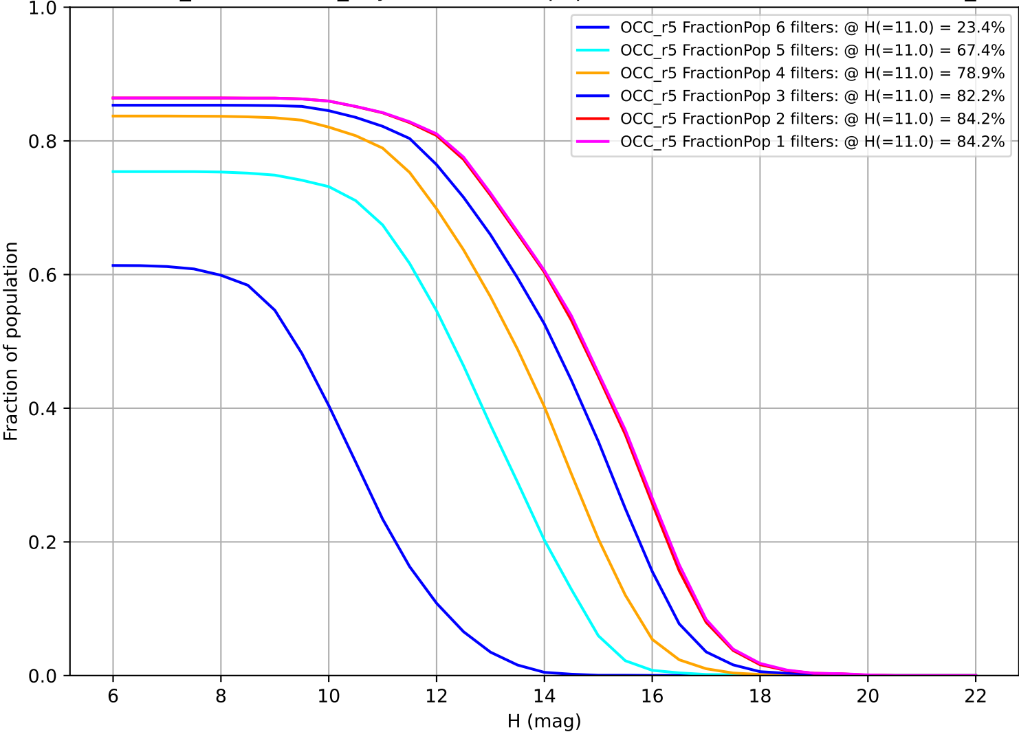
weather_cloudso2v3.5_10yrs: Fraction of population with colors in X filters OCC_r5
