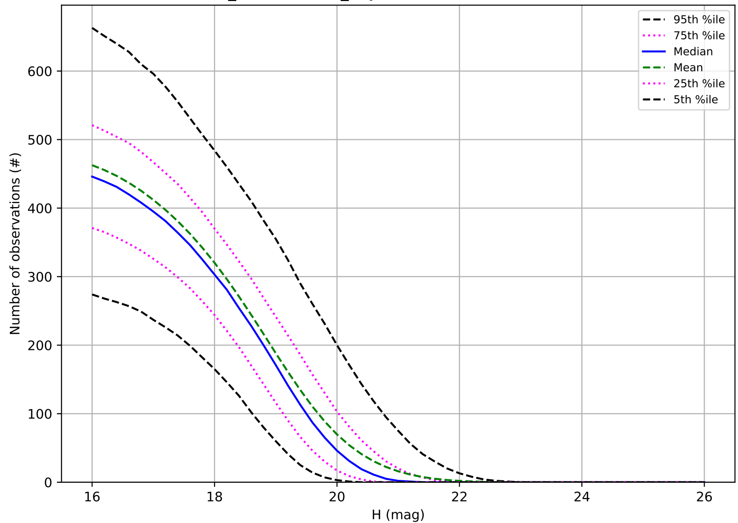
weather_cloudso2v3.5_10yrs: Number of observations MBA
