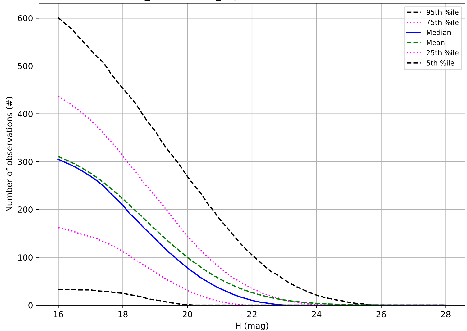
weather_cloudso2v3.5_10yrs: Number of observations NEO
