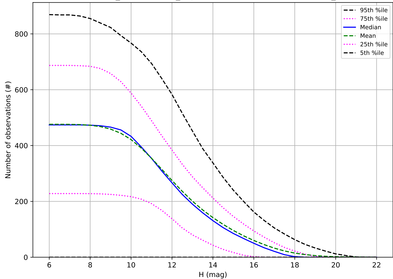
weather_cloudso2v3.5_10yrs: Number of observations OCC_r5
