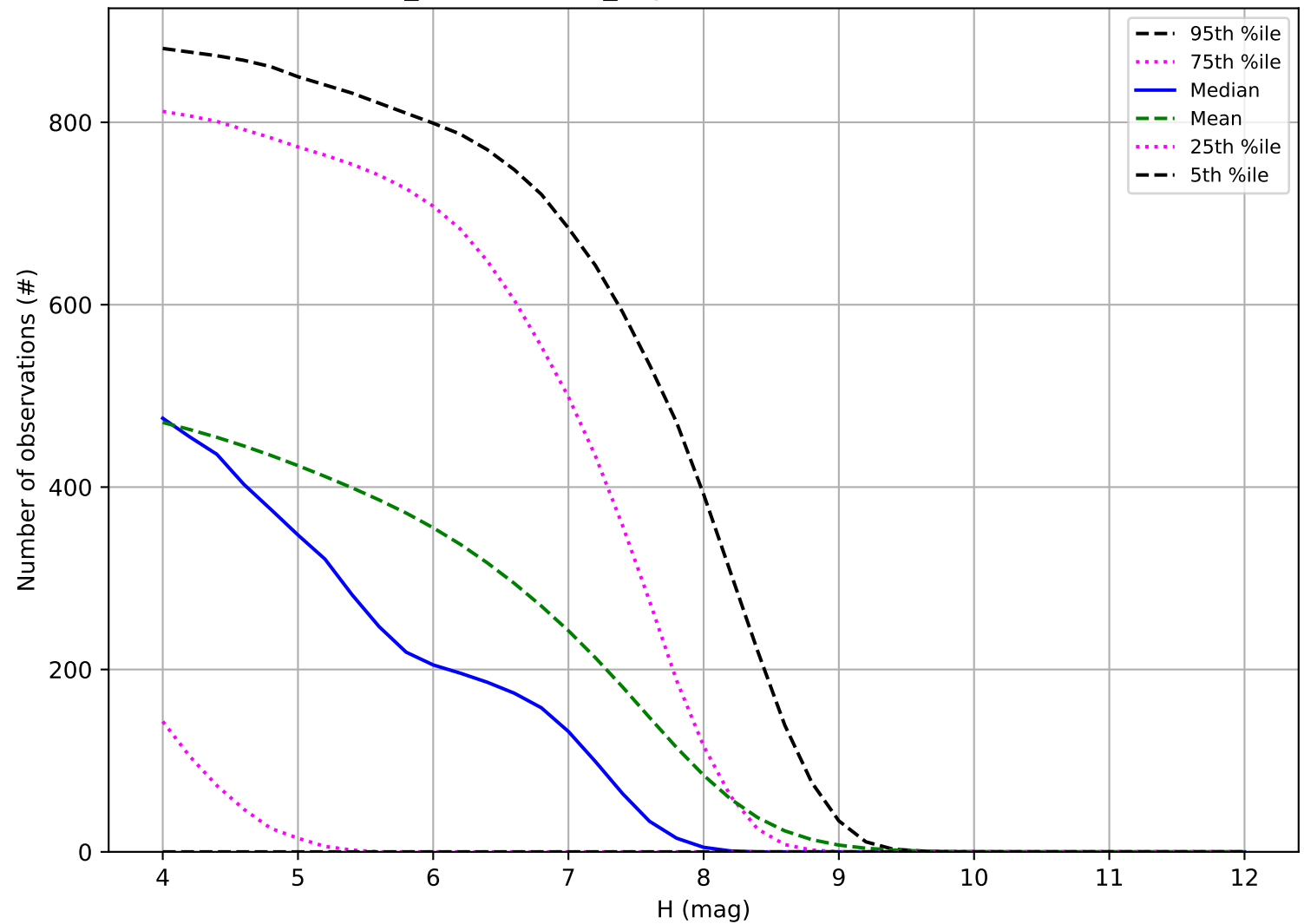
weather_cloudso2v3.5_10yrs: Number of observations TNO
