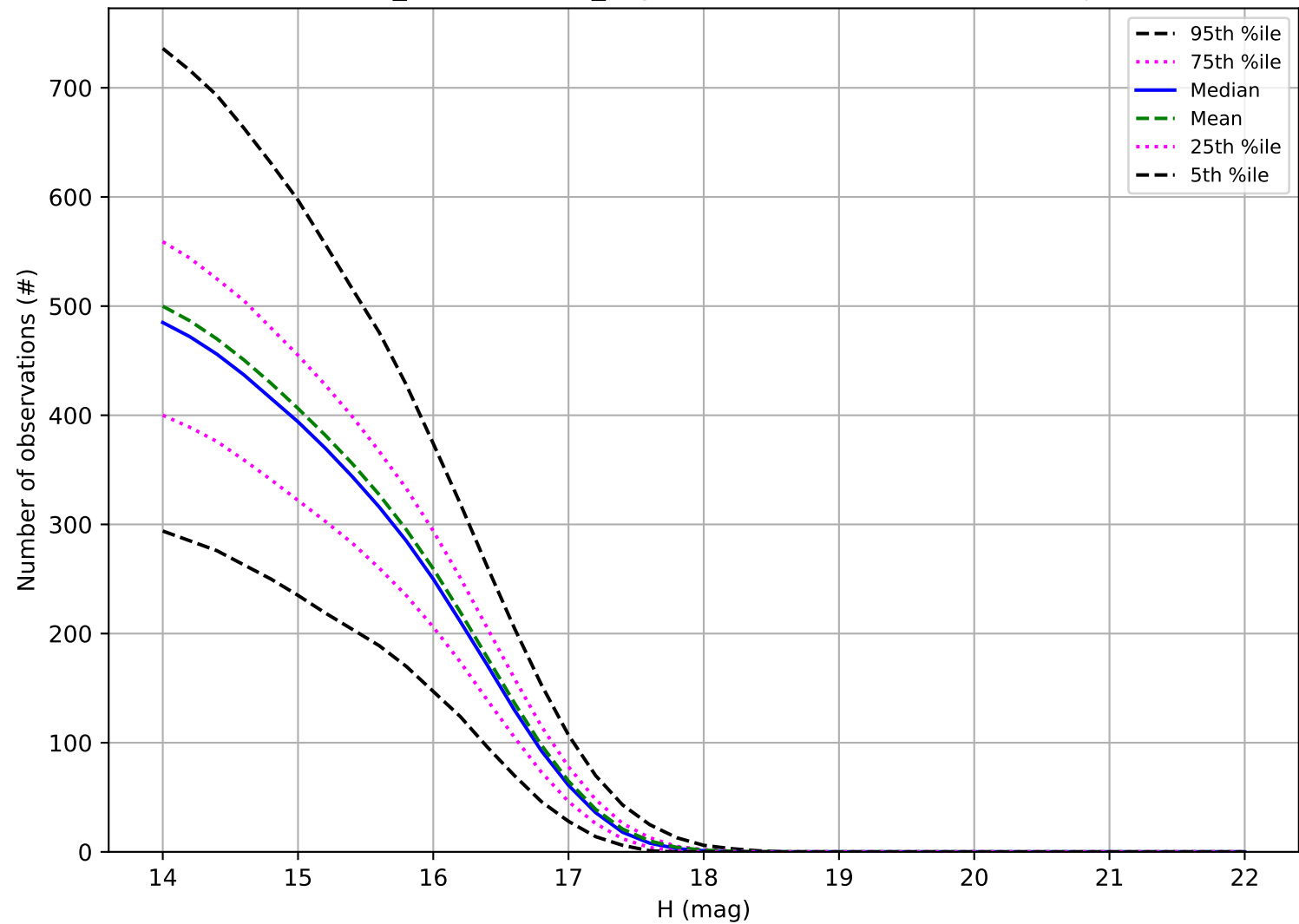
weather_cloudso2v3.5_10yrs: Number of observations Trojan
