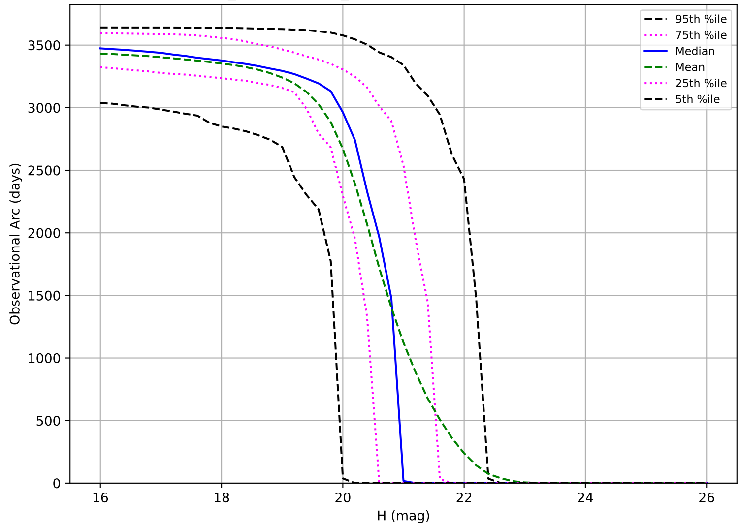
weather_cloudso2v3.5_10yrs: Observational Arc Length MBA
