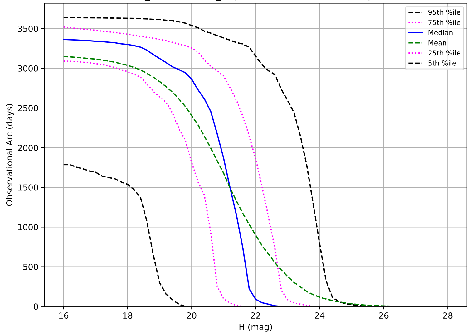
weather_cloudso2v3.5_10yrs: Observational Arc Length NEO
