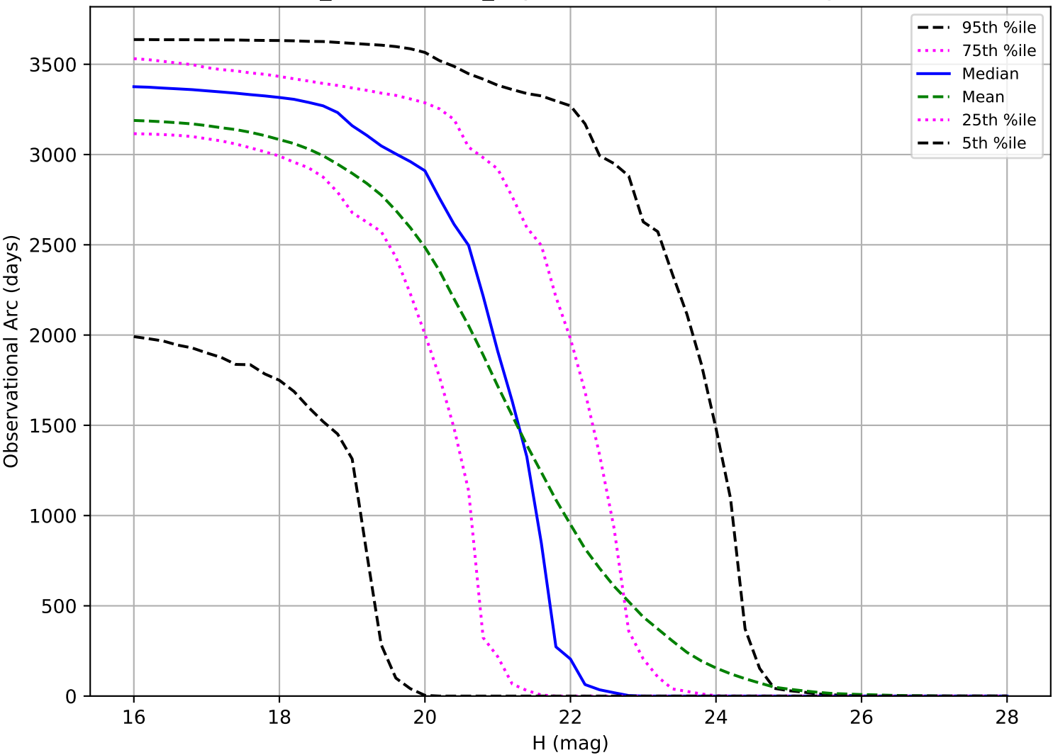
weather_cloudso2v3.5_10yrs: Observational Arc Length PHA
