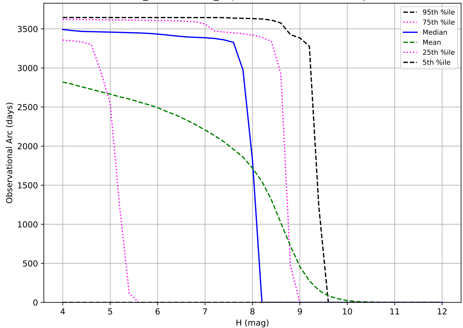
weather_cloudso2v3.5_10yrs: Observational Arc Length TNO
