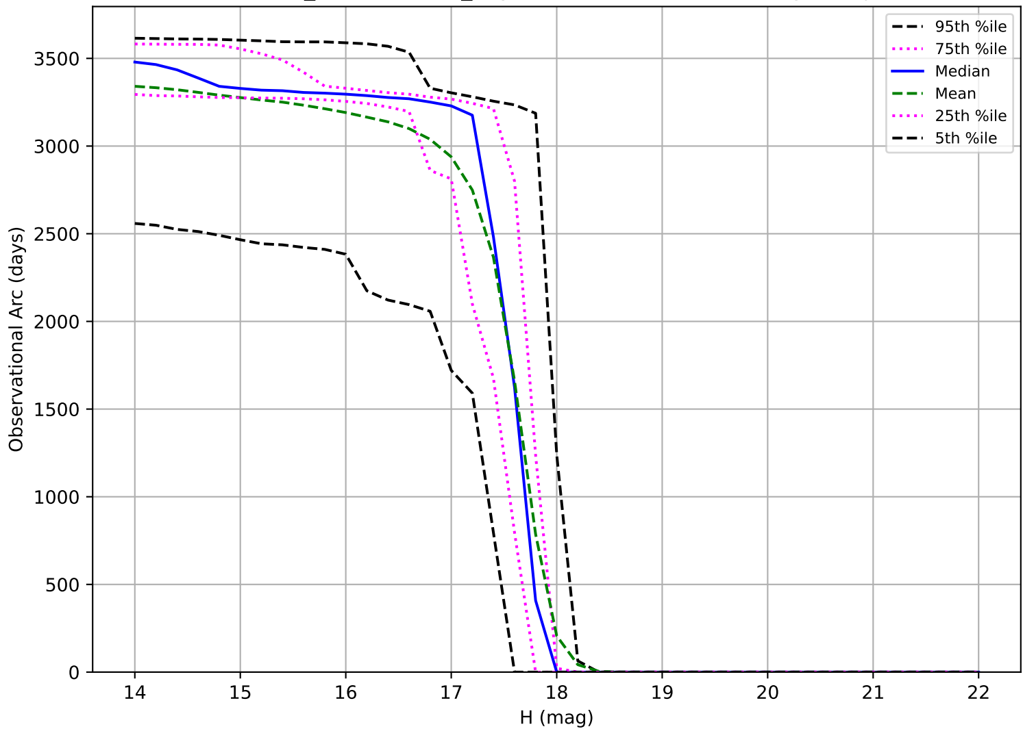
weather_cloudso2v3.5_10yrs: Observational Arc Length Trojan
