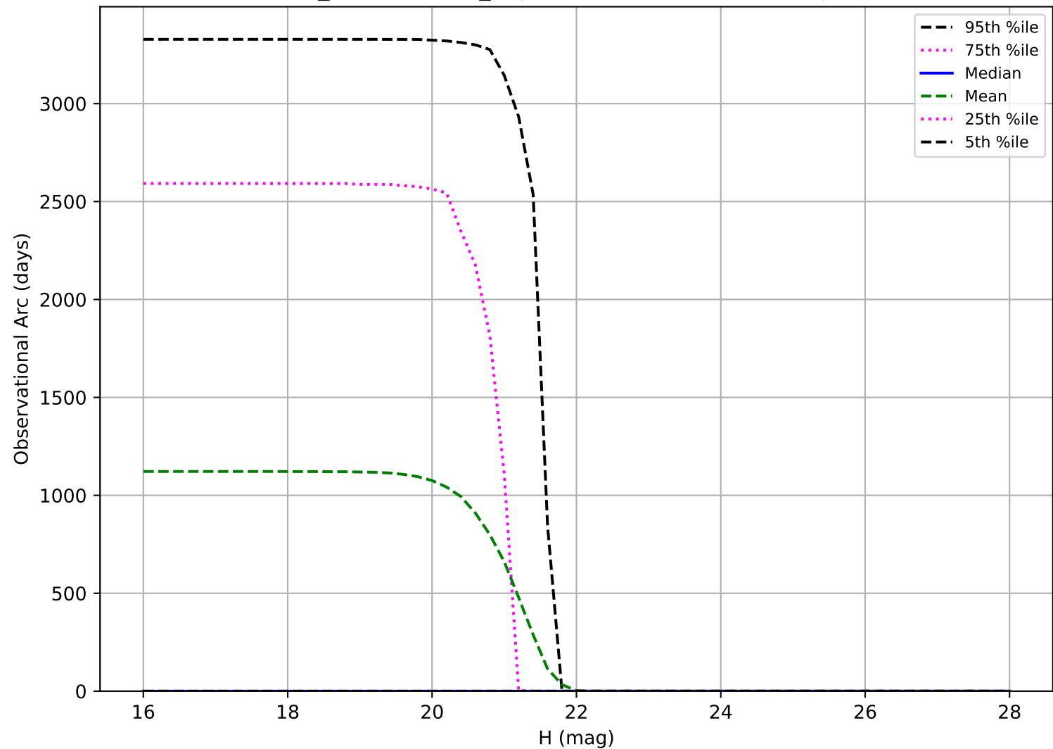
weather_cloudso2v3.5_10yrs: Observational Arc Length Vatira
