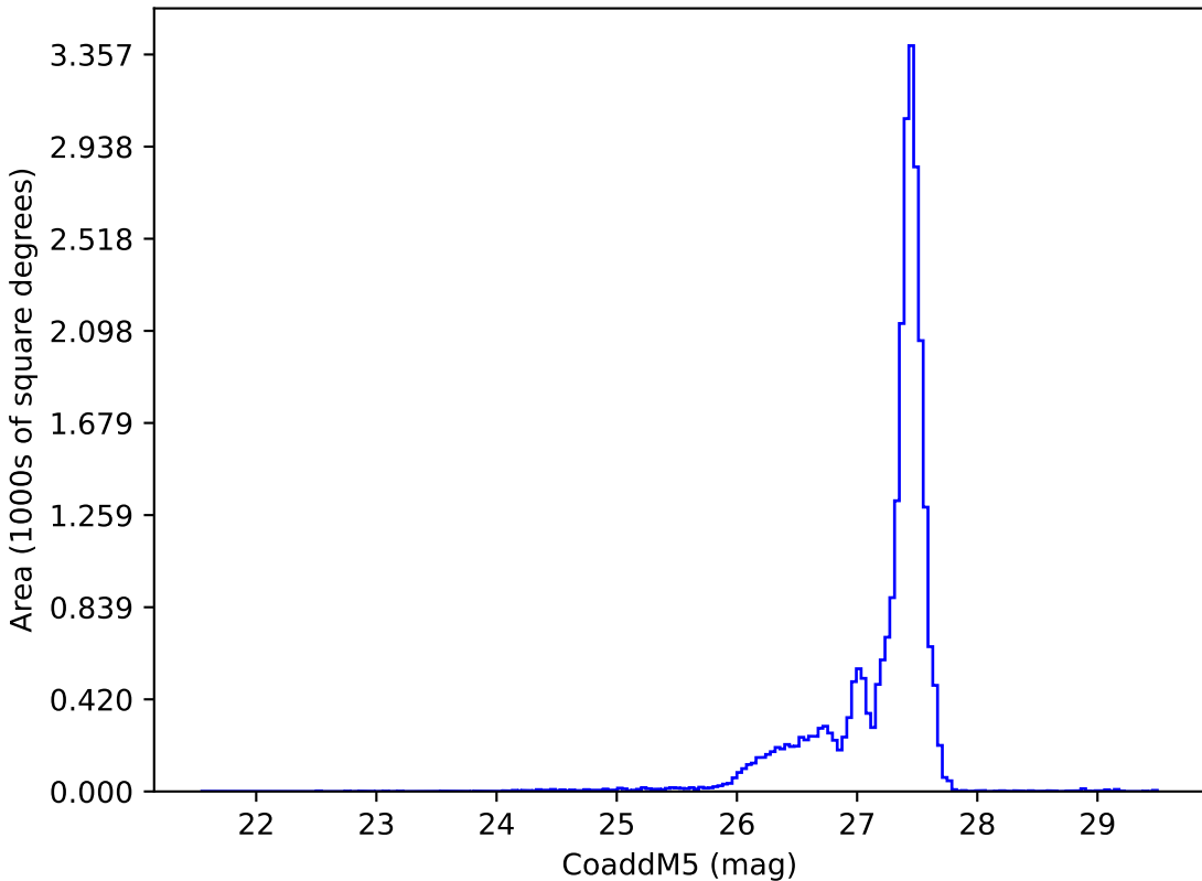
weather_cloudso30v3.5_10yrs : CoaddM5
