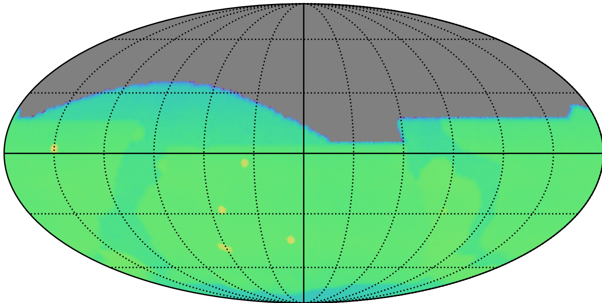
weather_cloudso30v3.5_10yrs : CoaddM5
