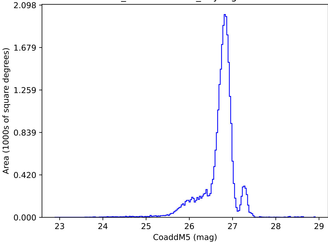
weather_cloudso30v3.5_10yrs g: CoaddM5
