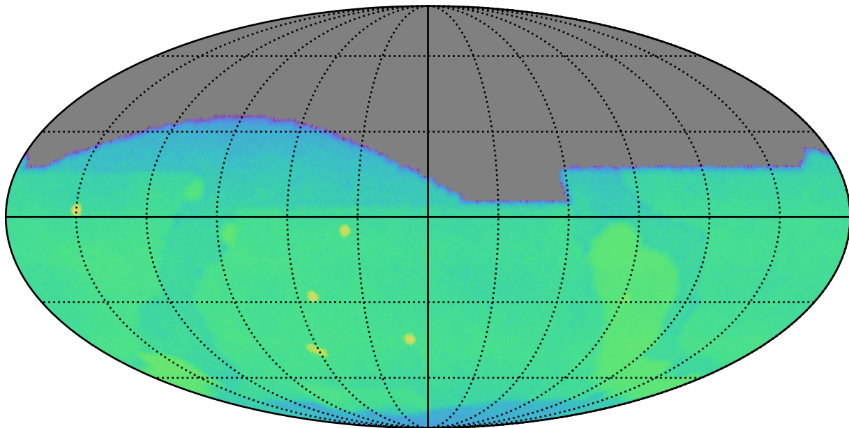
weather_cloudso30v3.5_10yrs g: CoaddM5
