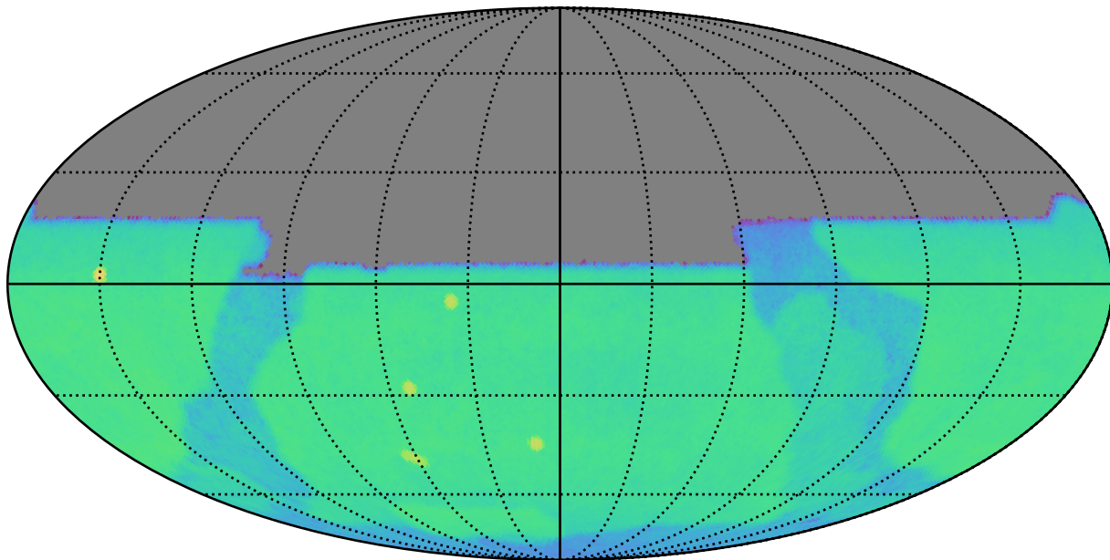
weather_cloudso30v3.5_10yrs u: CoaddM5
