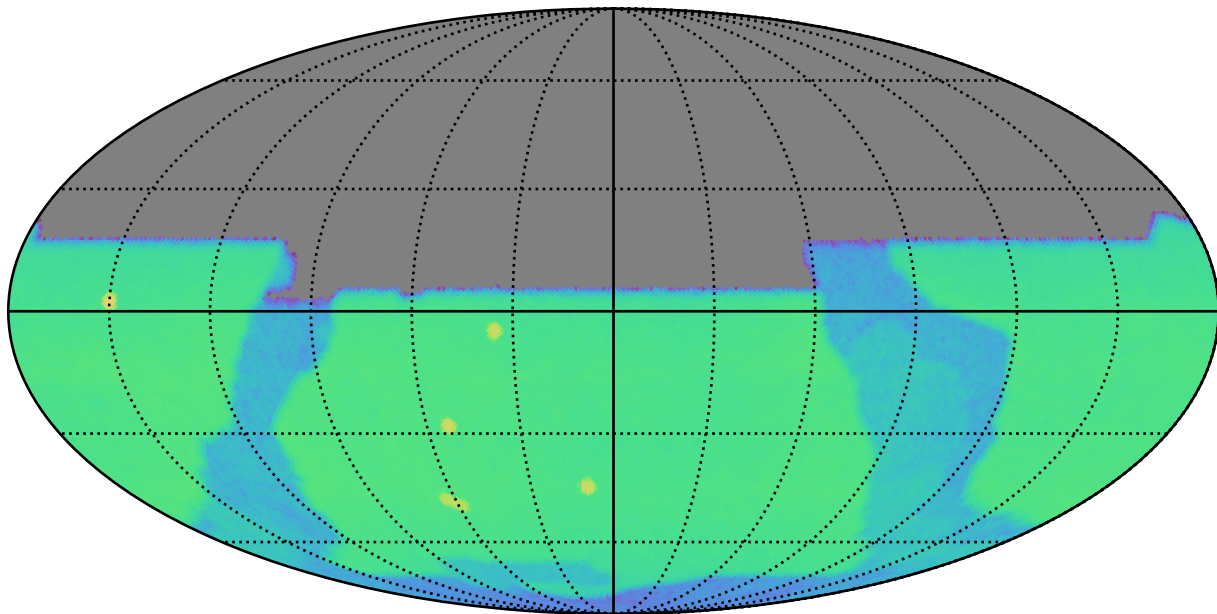
weather_cloudso30v3.5_10yrs y: CoaddM5
