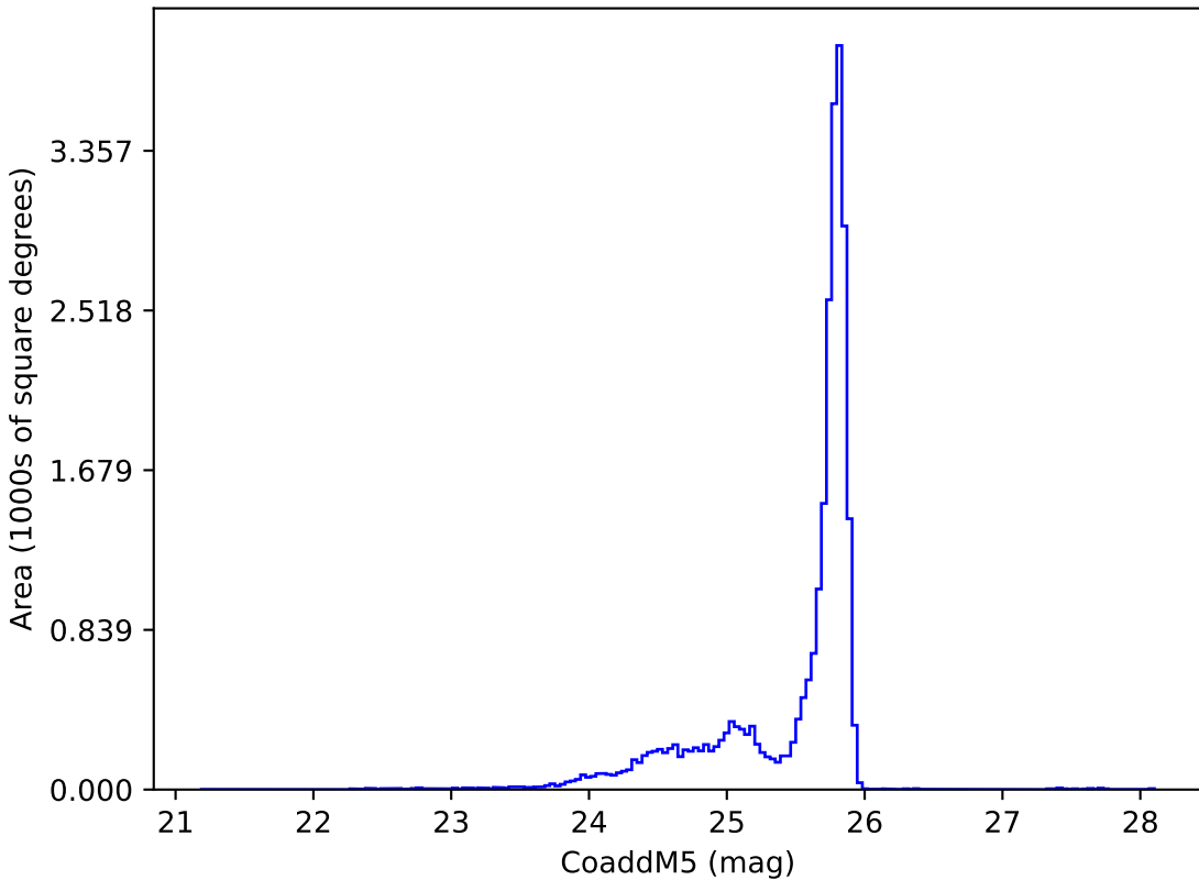
weather_cloudso30v3.5_10yrs z: CoaddM5
