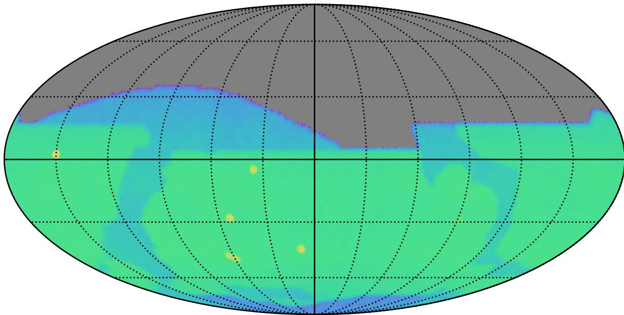
weather_cloudso30v3.5_10yrs z: CoaddM5
