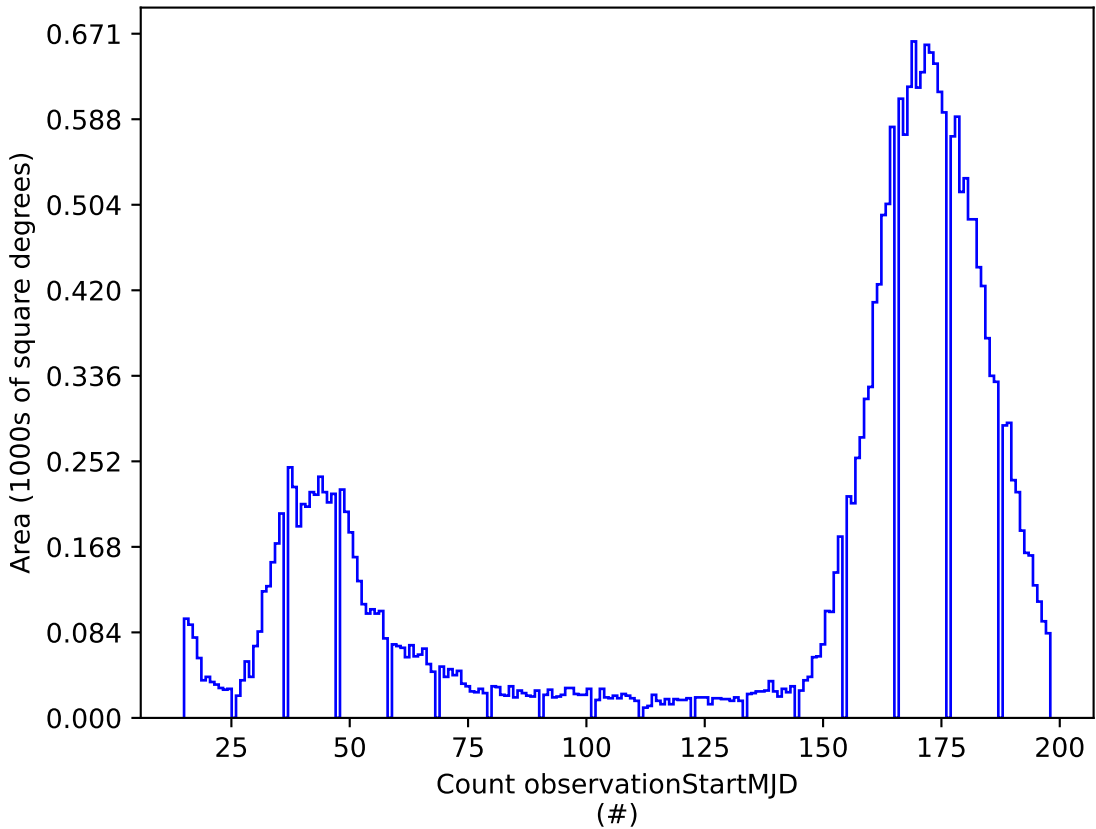
weather_cloudso30v3.5_10yrs z: Count observationStartMJD
