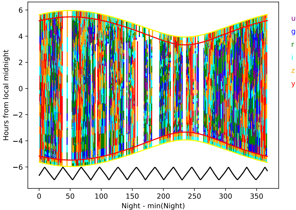
weather_cloudso30v3.5_10yrs year 3-4: Hourglass
