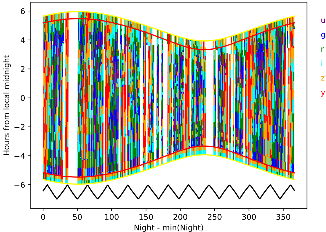
weather_cloudso30v3.5_10yrs year 6-7: Hourglass
