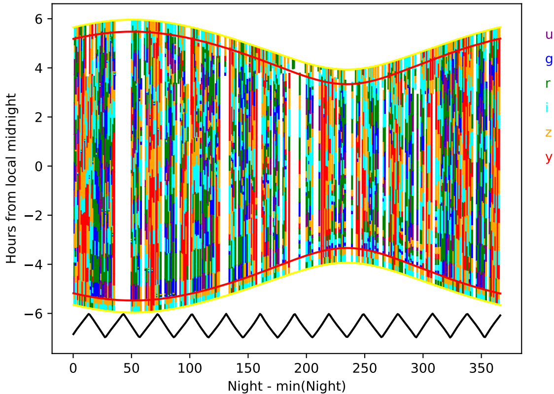
weather_cloudso30v3.5_10yrs year 8-9: Hourglass
