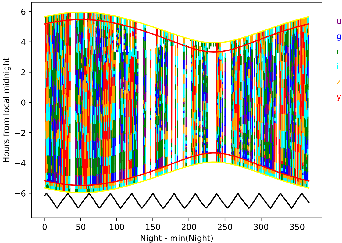
weather_cloudso30v3.5_10yrs year 9-10: Hourglass
