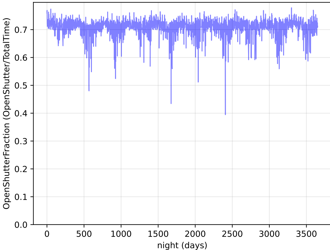
weather_cloudso30v3.5_10yrs : OpenShutterFraction
