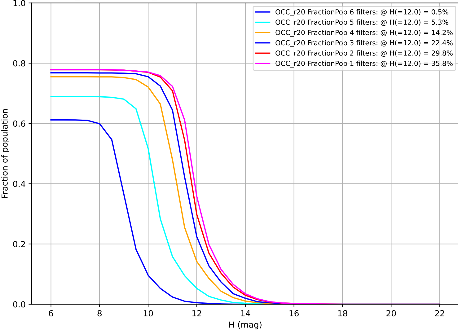
weather_cloudso30v3.5_10yrs: Fraction of population with colors in X filters OCC_r20
