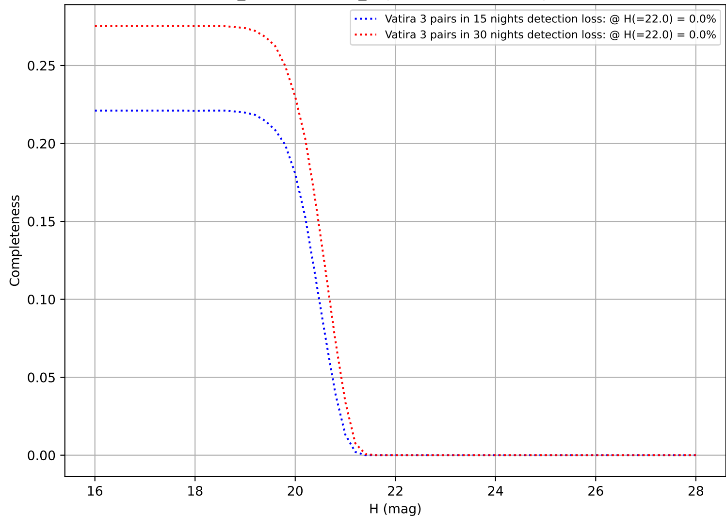
weather_cloudso30v3.5_10yrs: DifferentialCompleteness
