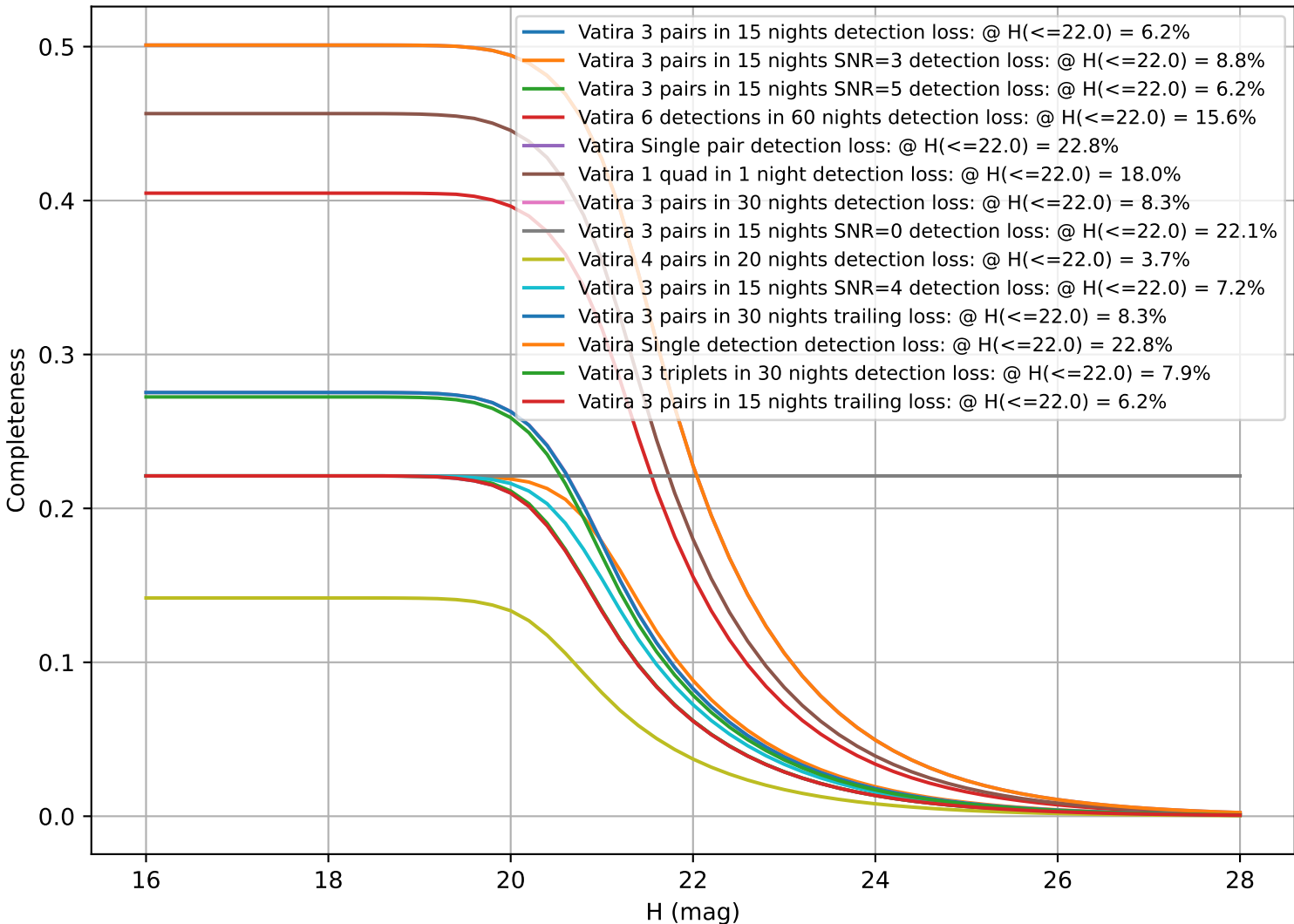
weather_cloudso30v3.5_10yrs: CumulativeCompleteness
