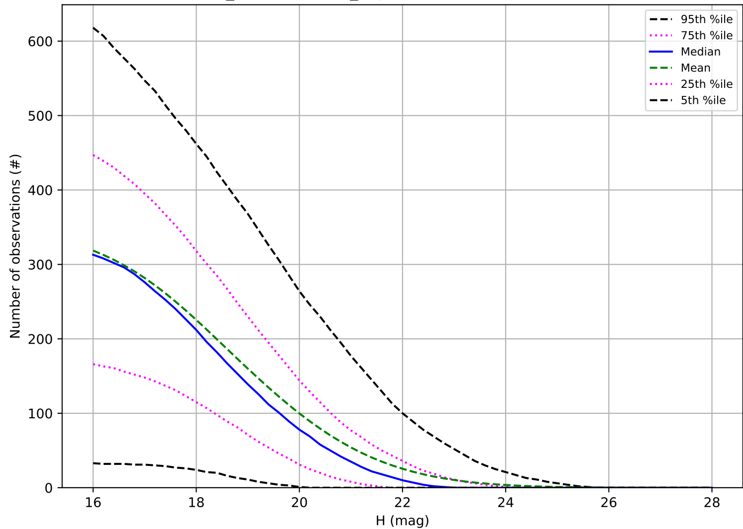
weather_cloudso30v3.5_10yrs: Number of observations NEO
