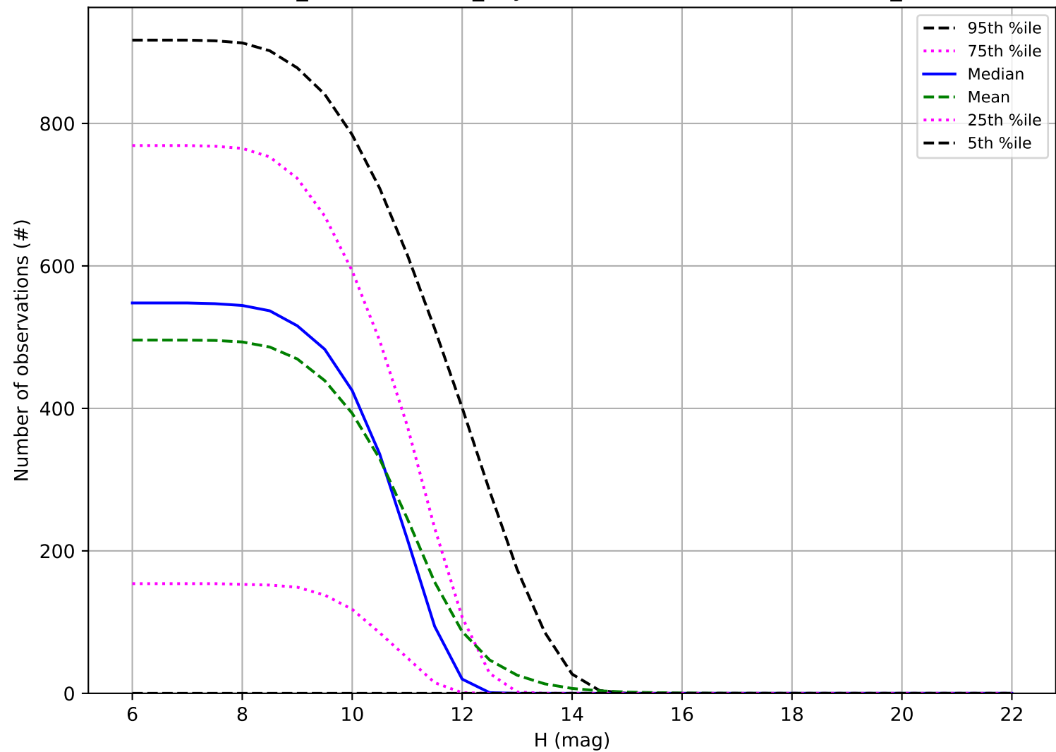
weather_cloudso30v3.5_10yrs: Number of observations OCC_r20
