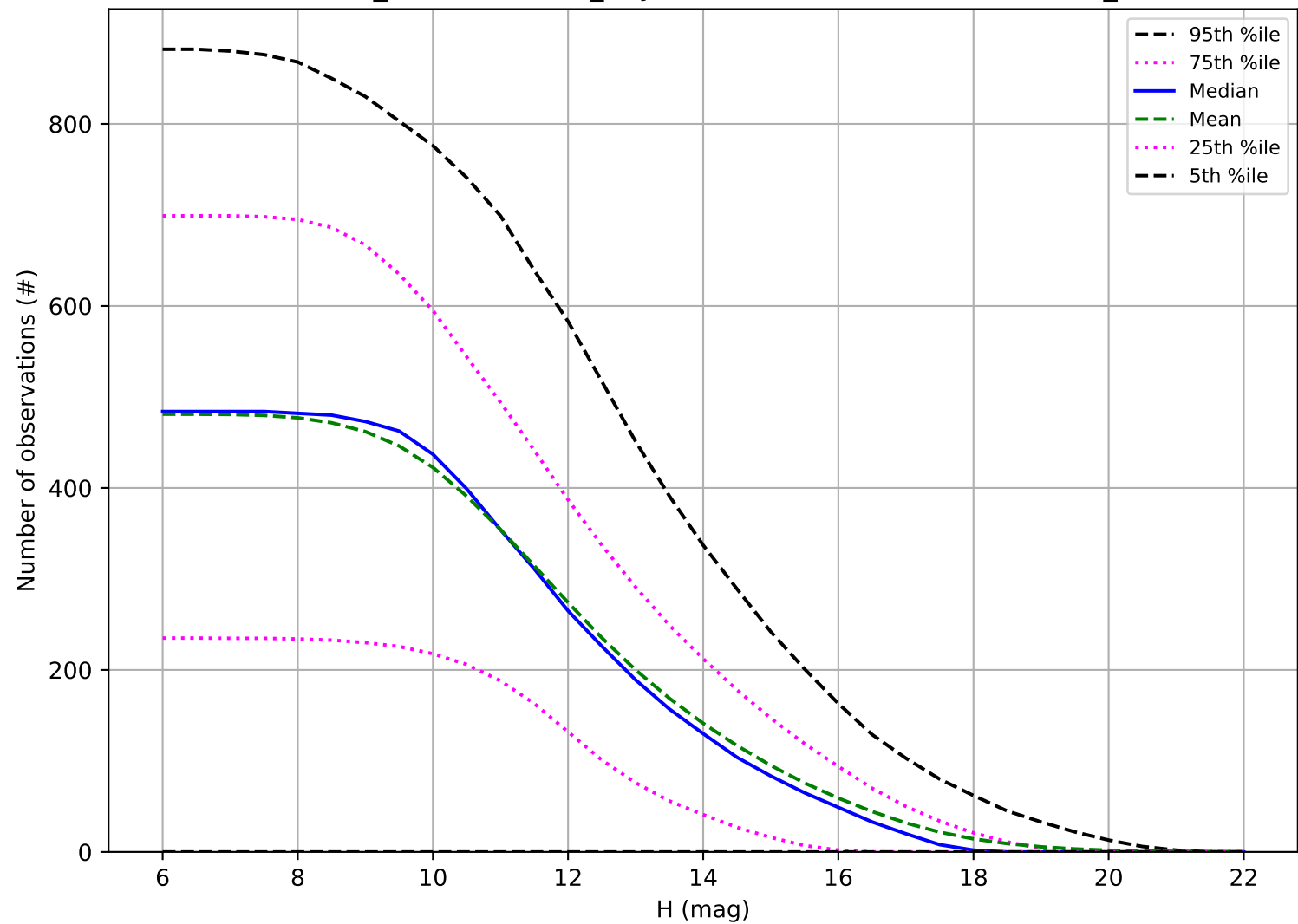
weather_cloudso30v3.5_10yrs: Number of observations OCC_r5
