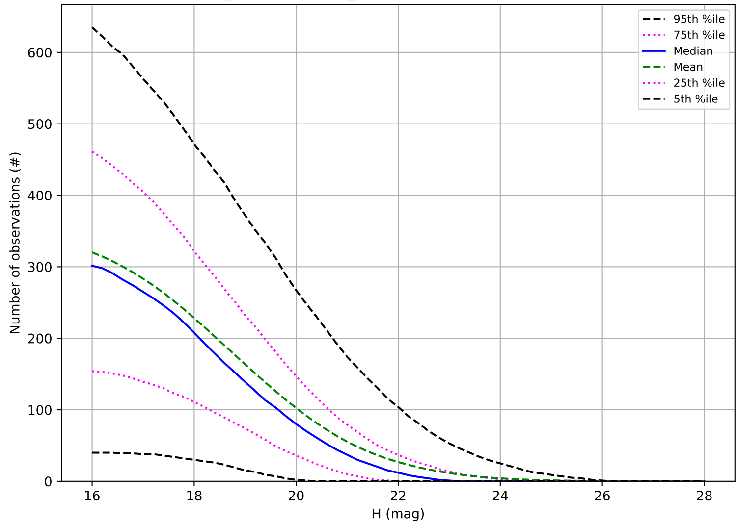
weather_cloudso30v3.5_10yrs: Number of observations PHA
