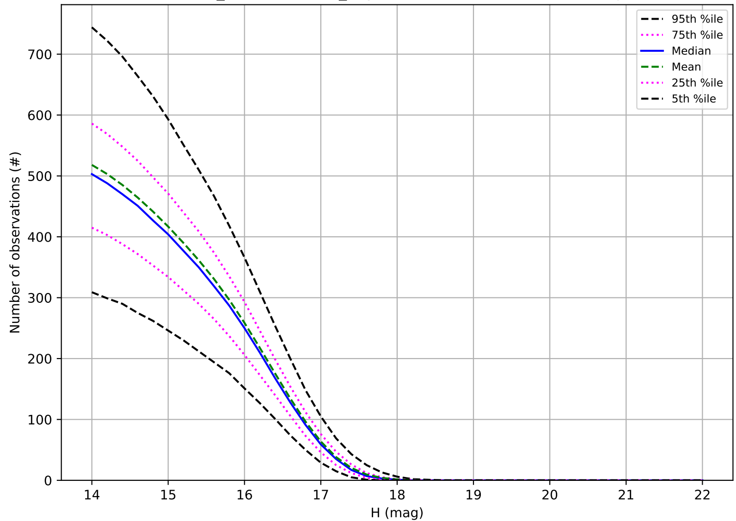
weather_cloudso30v3.5_10yrs: Number of observations Trojan
