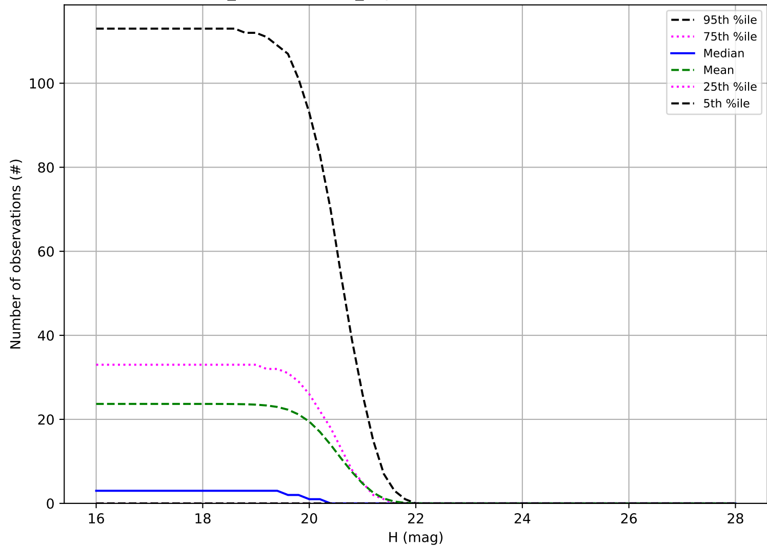
weather_cloudso30v3.5_10yrs: Number of observations Vatira
