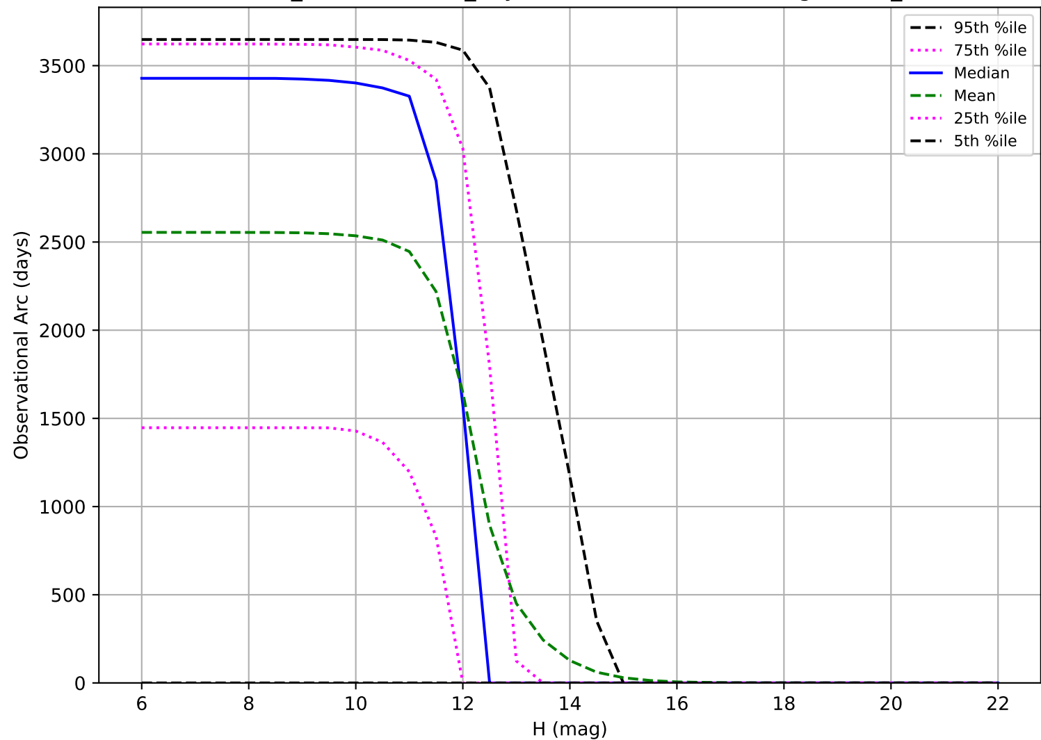
weather_cloudso30v3.5_10yrs: Observational Arc Length OCC_r20
