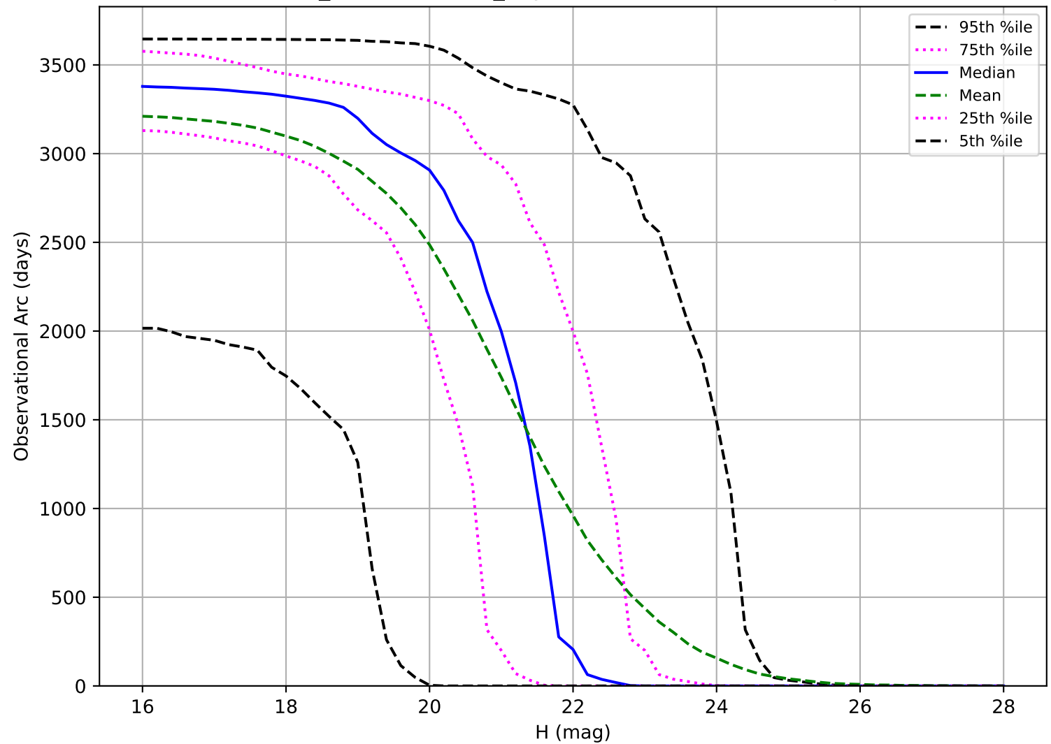
weather_cloudso30v3.5_10yrs: Observational Arc Length PHA
