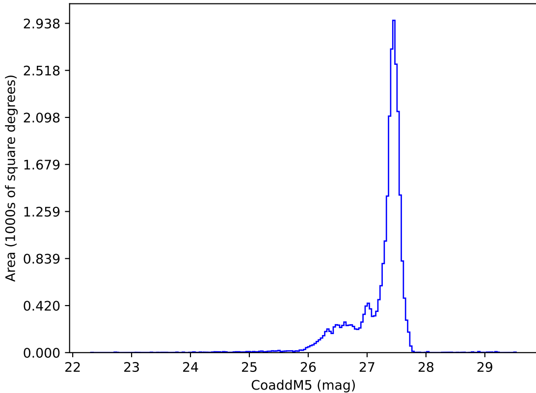
weather_cloudso31v3.5_10yrs : CoaddM5
