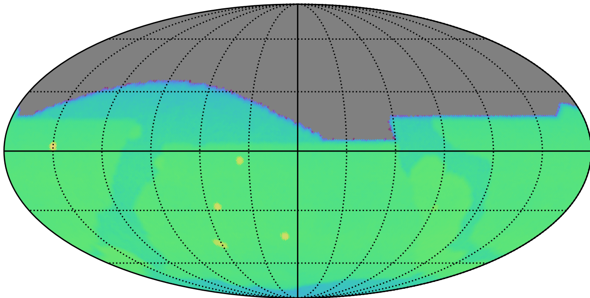
weather_cloudso31v3.5_10yrs : CoaddM5
