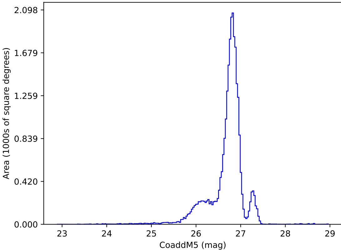
weather_cloudso31v3.5_10yrs g: CoaddM5
