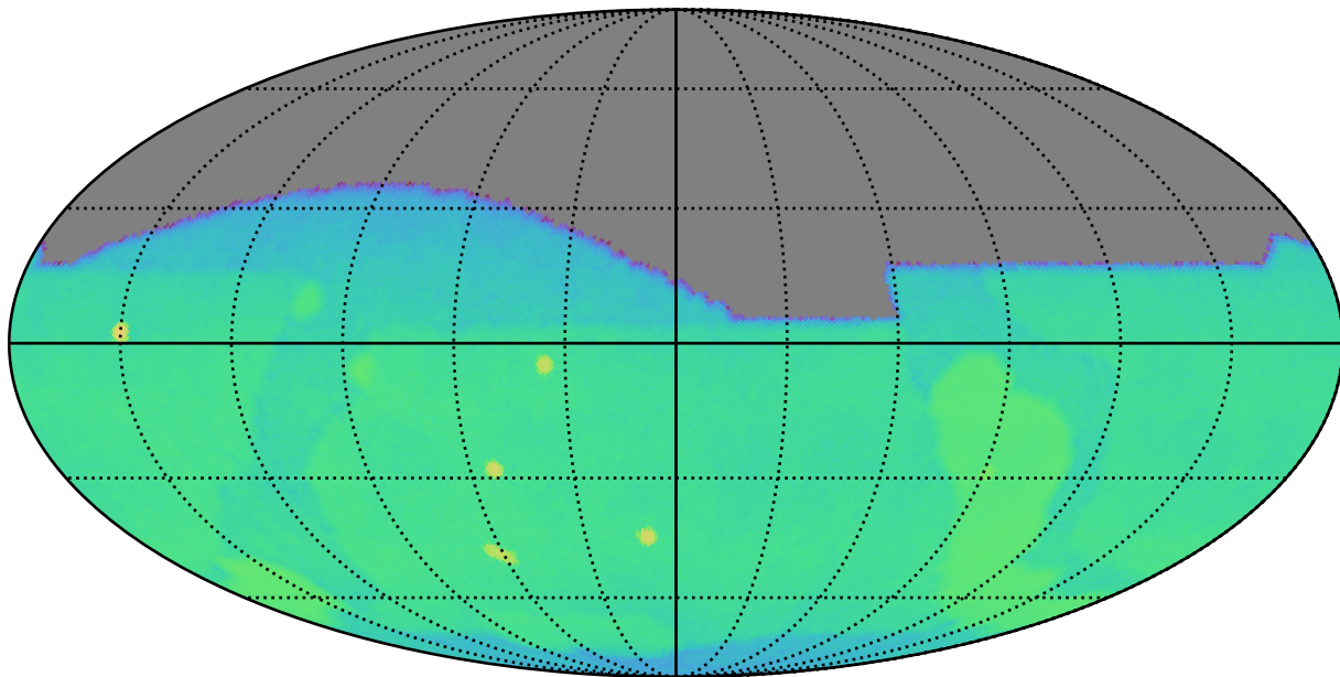
weather_cloudso31v3.5_10yrs g: CoaddM5
