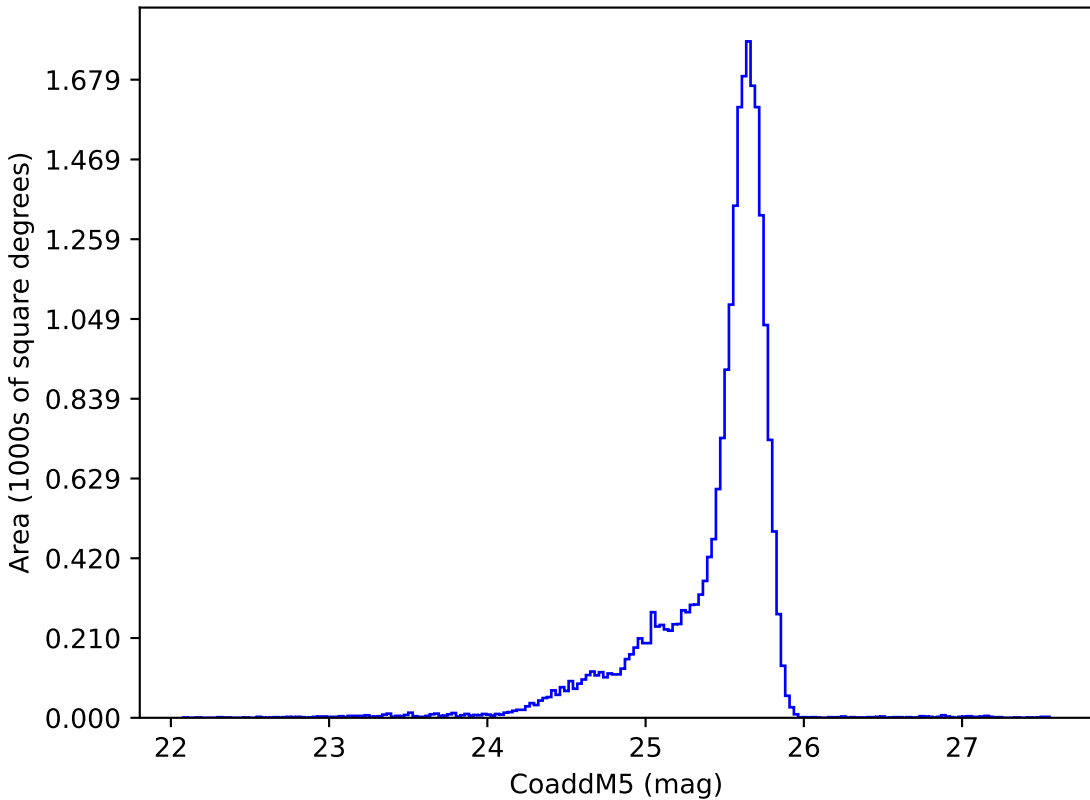
weather_cloudso31v3.5_10yrs u: CoaddM5
