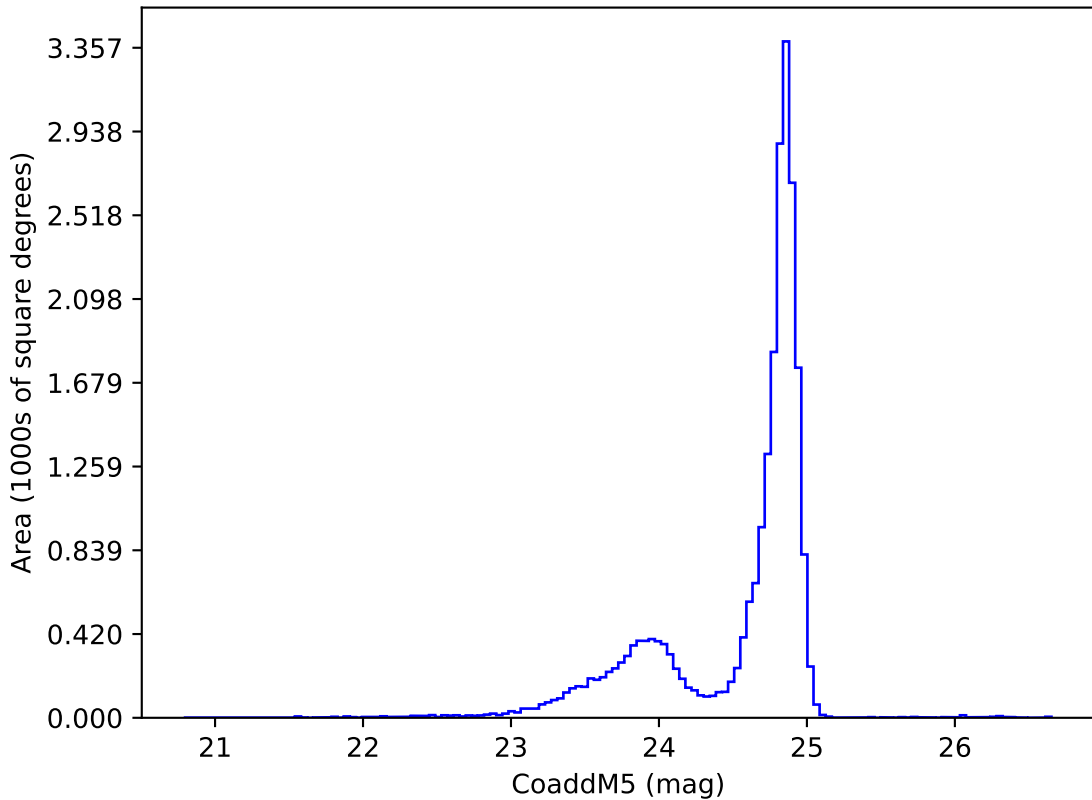
weather_cloudso31v3.5_10yrs y: CoaddM5
