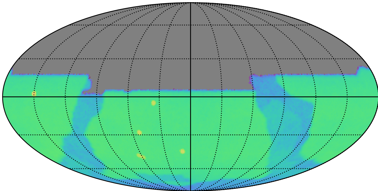
weather_cloudso31v3.5_10yrs y: CoaddM5
