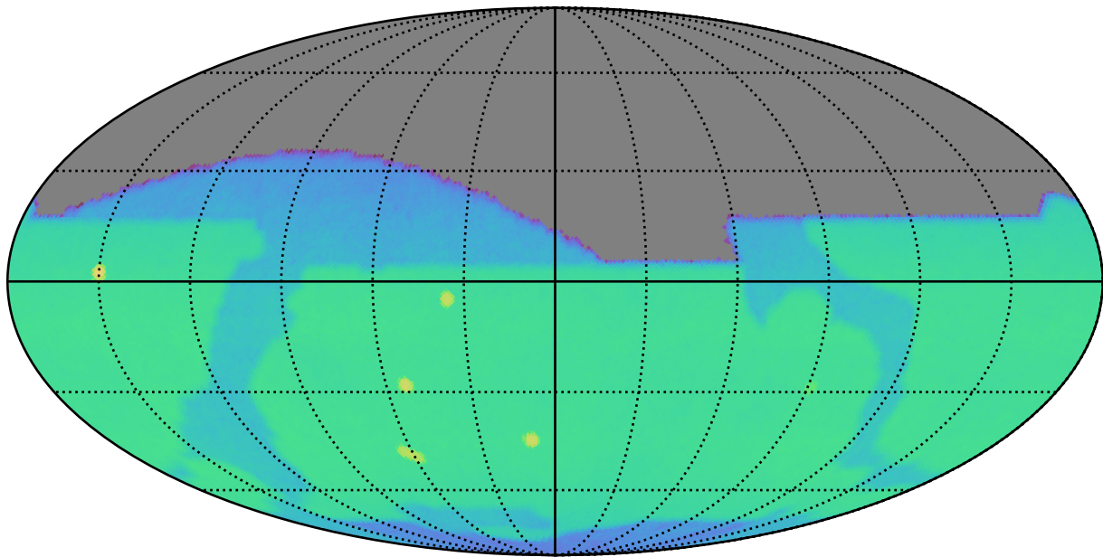
weather_cloudso31v3.5_10yrs z: CoaddM5
