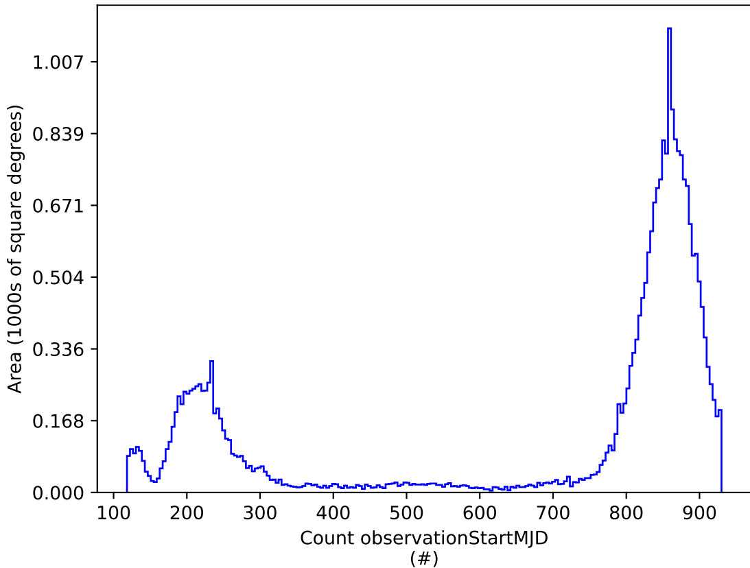
weather_cloudso31v3.5_10yrs : Count observationStartMJD
