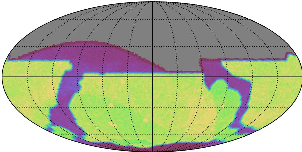
weather_cloudso31v3.5_10yrs : Count observationStartMJD
