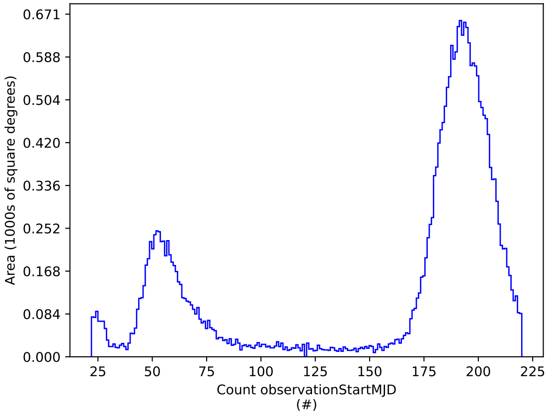
weather_cloudso31v3.5_10yrs i: Count observationStartMJD
